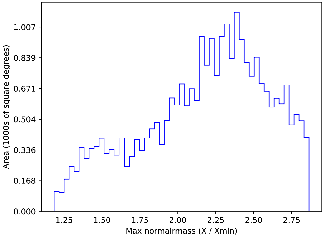
weather_cloudso35v3.4_10yrs All sky z band: Max normairmass
