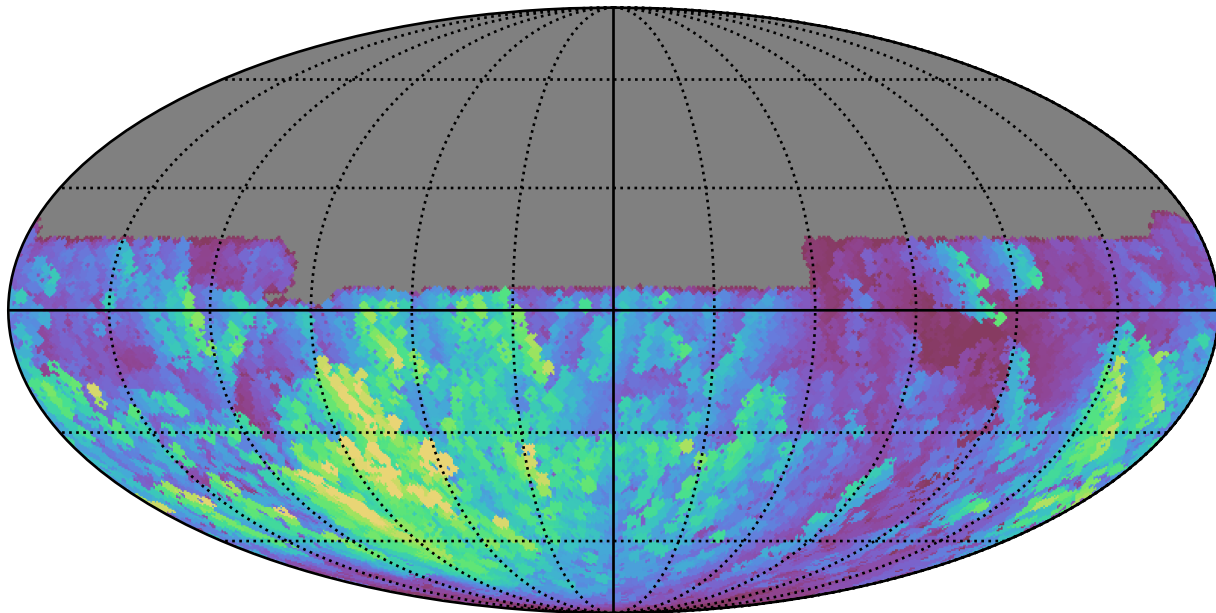
weather_cloudso35v3.4_10yrs All sky u band: Max normairmass
