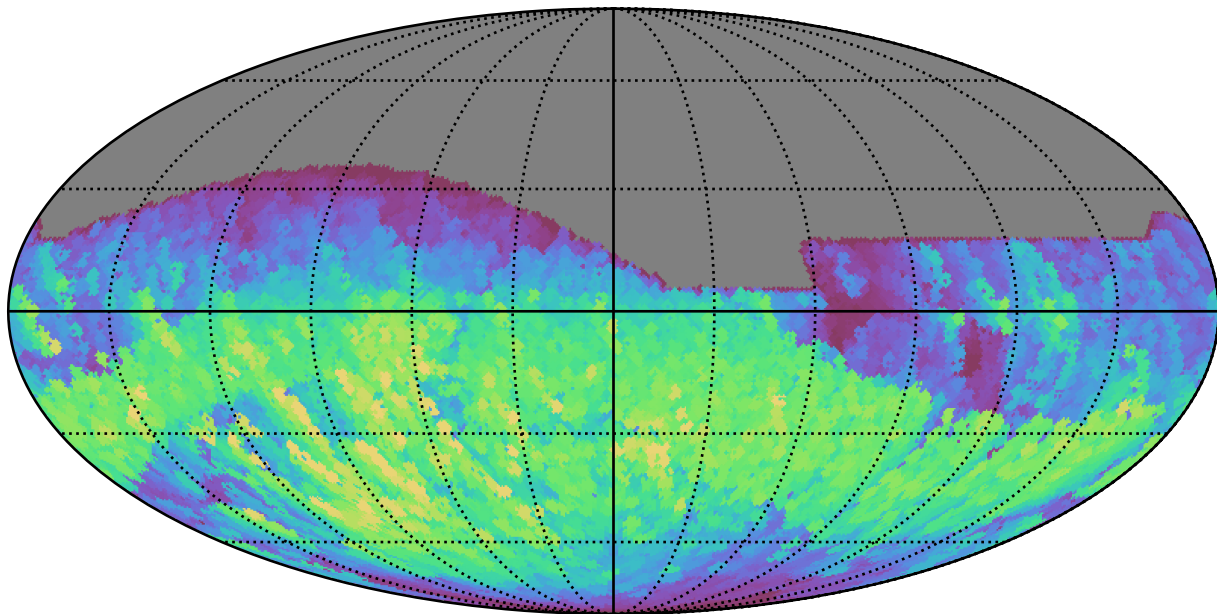
weather_cloudso35v3.4_10yrs All sky r band: Max normairmass
