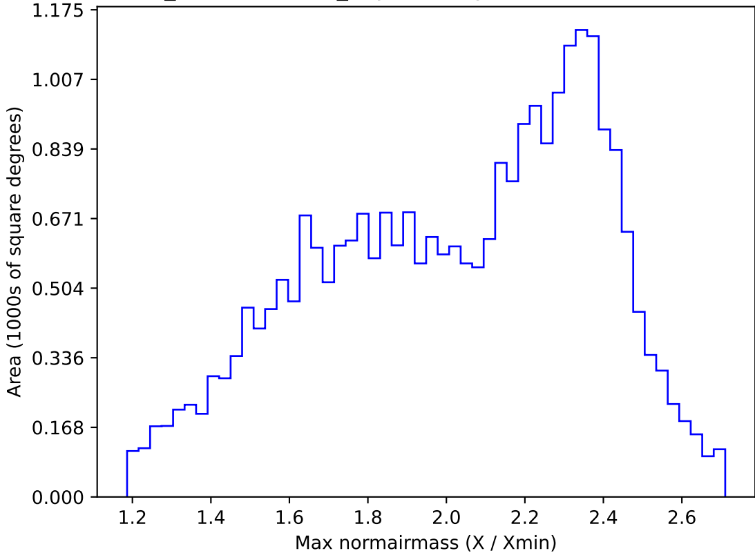
weather_cloudso35v3.4_10yrs All sky r band: Max normairmass
