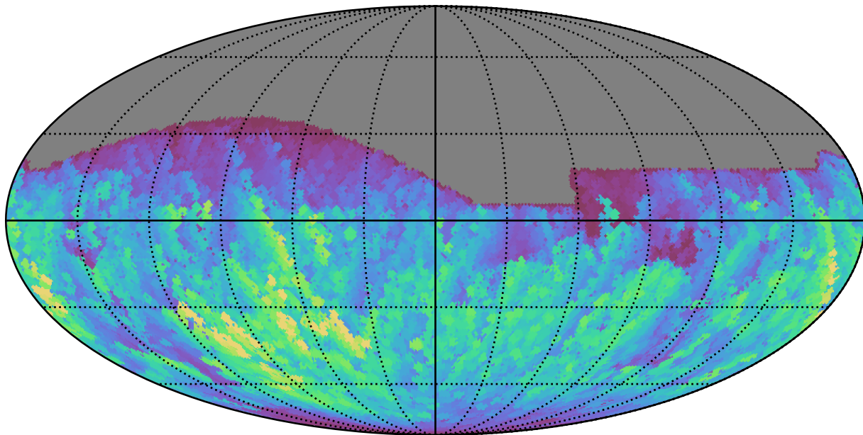
weather_cloudso35v3.4_10yrs All sky g band: Max normairmass
