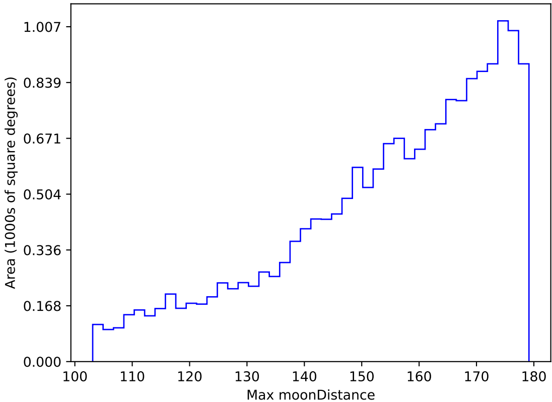
weather_cloudso35v3.4_10yrs WFD z band: Max moonDistance
