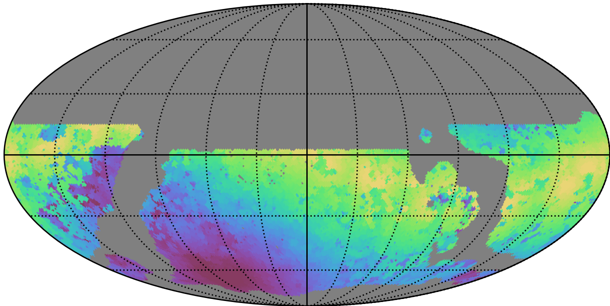
weather_cloudso35v3.4_10yrs WFD y band: Max moonDistance
