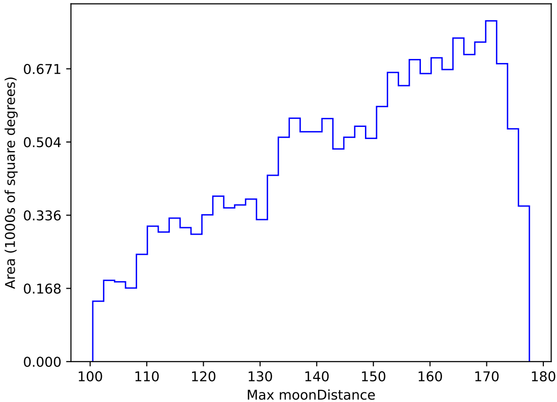
weather_cloudso35v3.4_10yrs WFD y band: Max moonDistance
