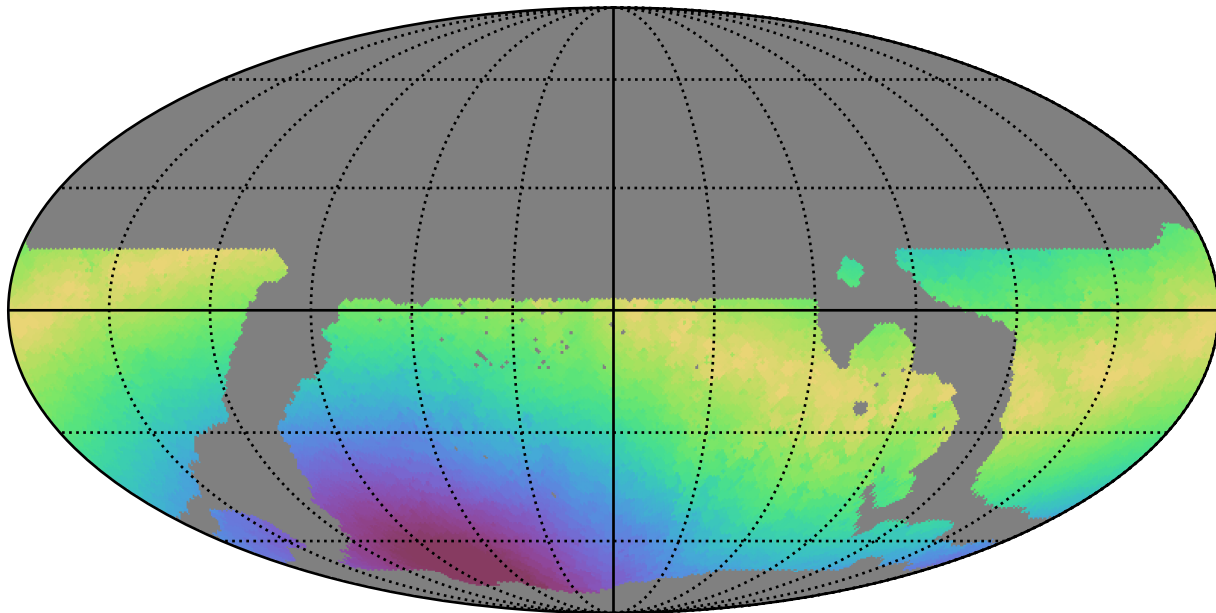
weather_cloudso35v3.4_10yrs WFD u band: Max moonDistance
