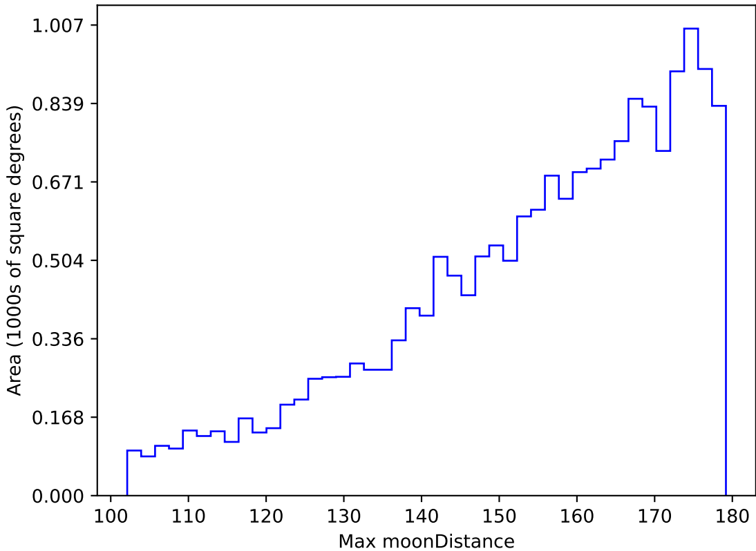
weather_cloudso35v3.4_10yrs WFD u band: Max moonDistance
