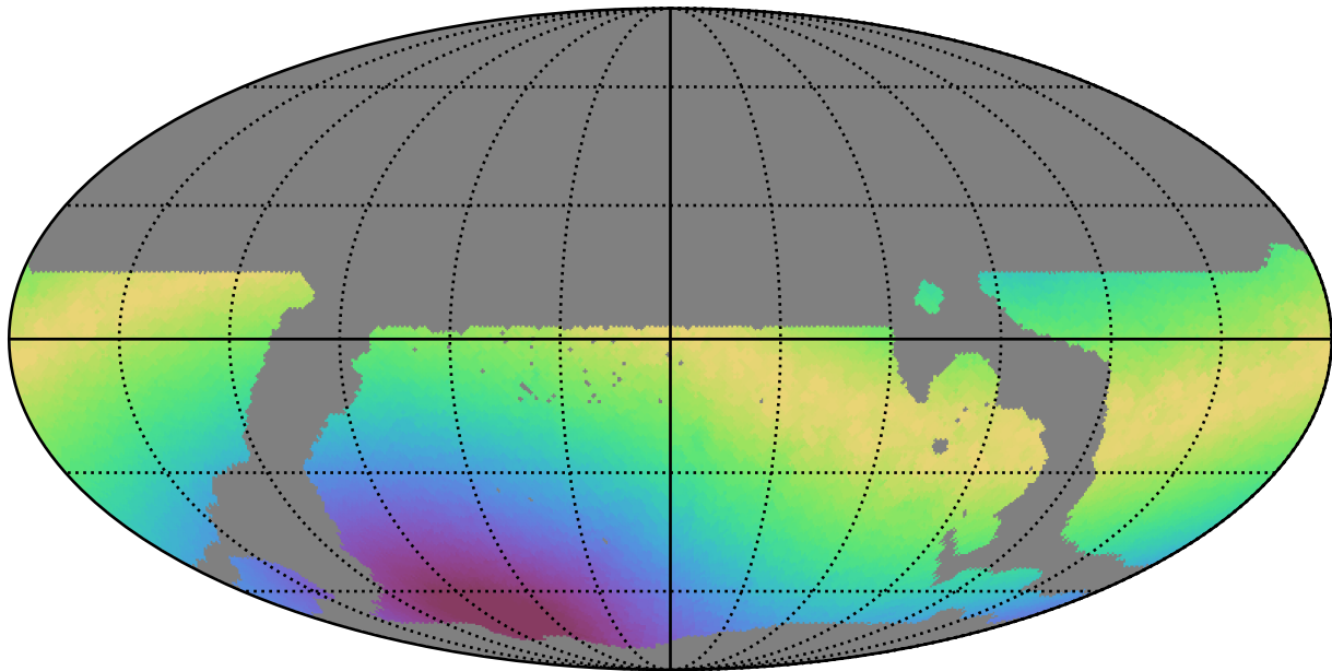
weather_cloudso35v3.4_10yrs WFD r band: Max moonDistance
