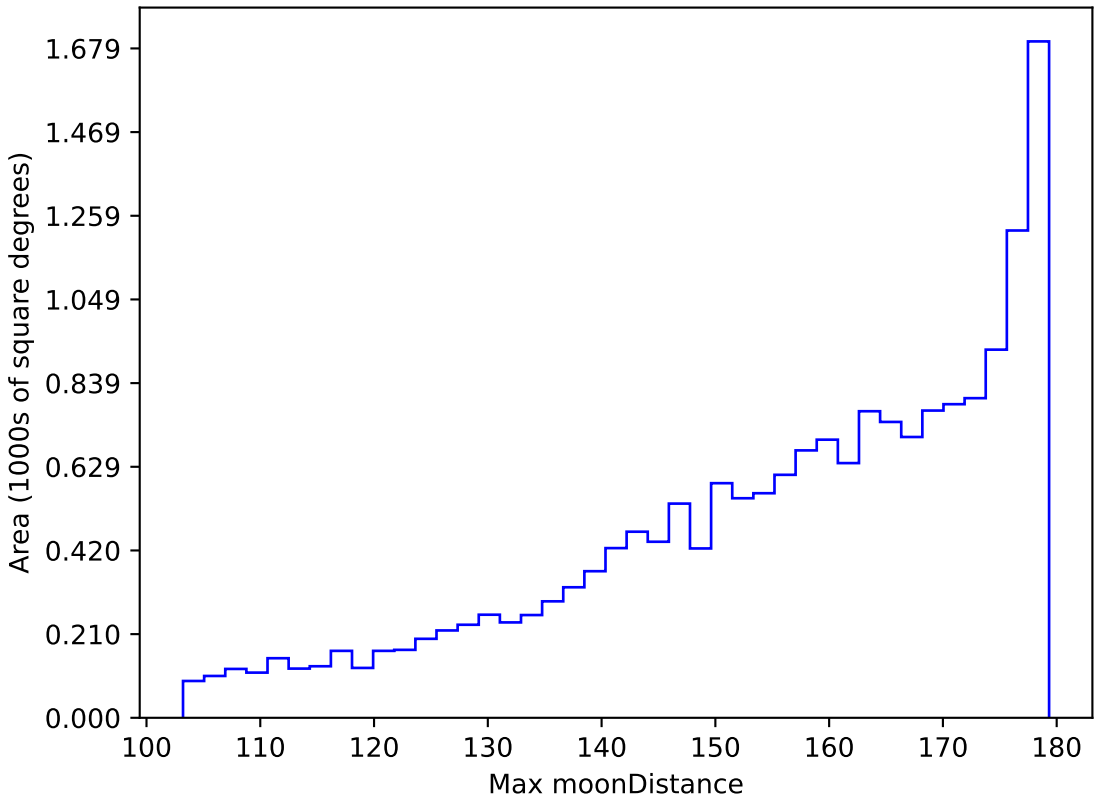
weather_cloudso35v3.4_10yrs WFD r band: Max moonDistance
