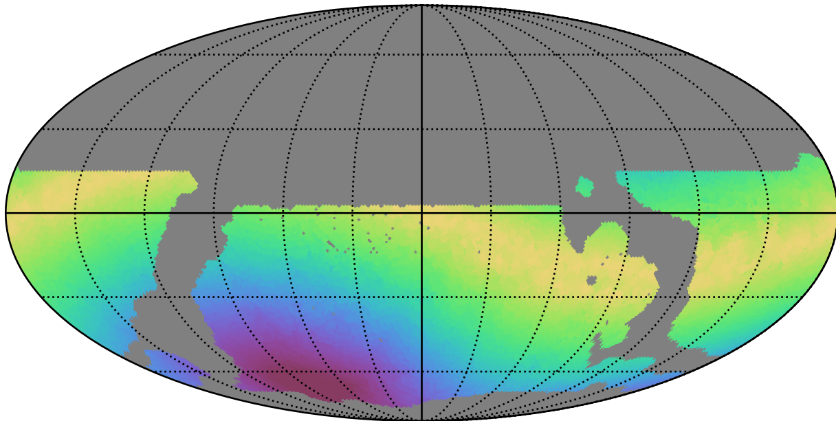
weather_cloudso35v3.4_10yrs WFD i band: Max moonDistance
