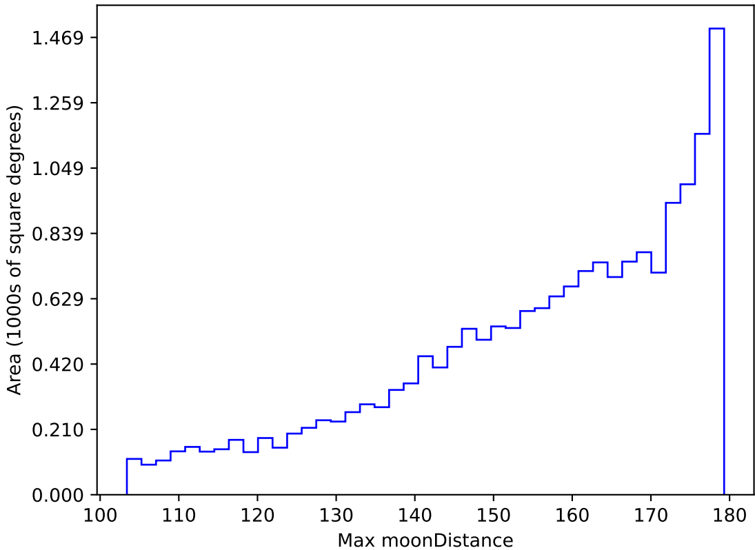
weather_cloudso35v3.4_10yrs WFD i band: Max moonDistance
