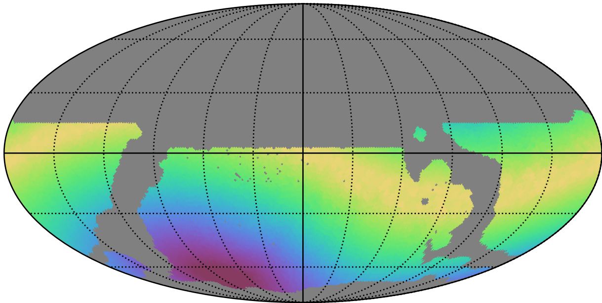
weather_cloudso35v3.4_10yrs WFD all bands: Max moonDistance
