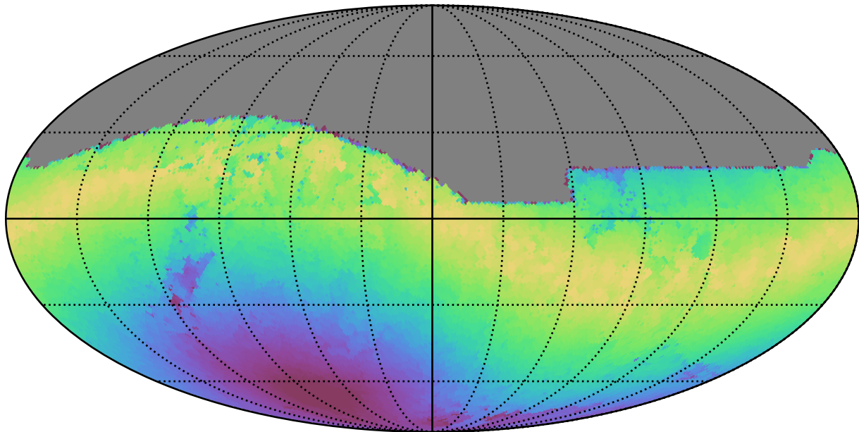
weather_cloudso35v3.4_10yrs All sky z band: Max moonDistance
