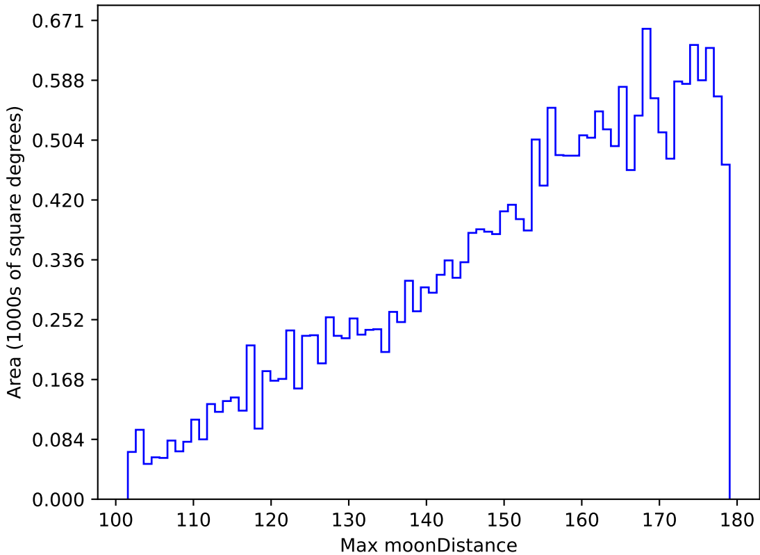
weather_cloudso35v3.4_10yrs All sky u band: Max moonDistance
