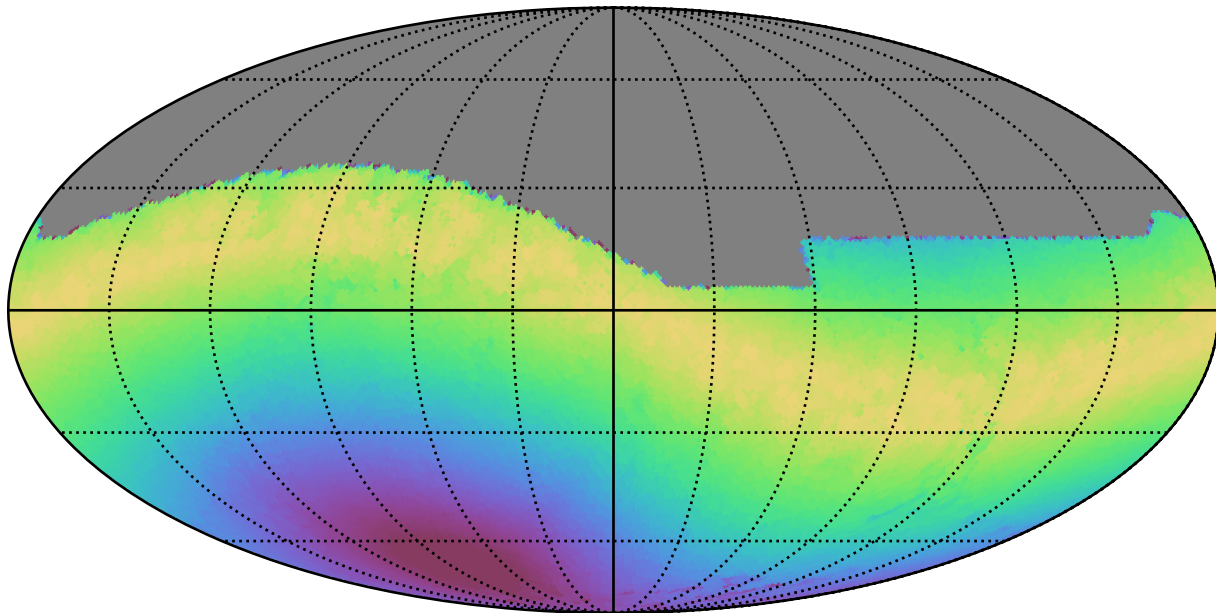
weather_cloudso35v3.4_10yrs All sky r band: Max moonDistance
