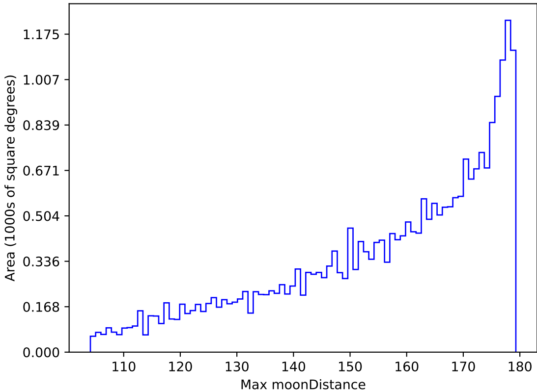
weather_cloudso35v3.4_10yrs All sky r band: Max moonDistance
