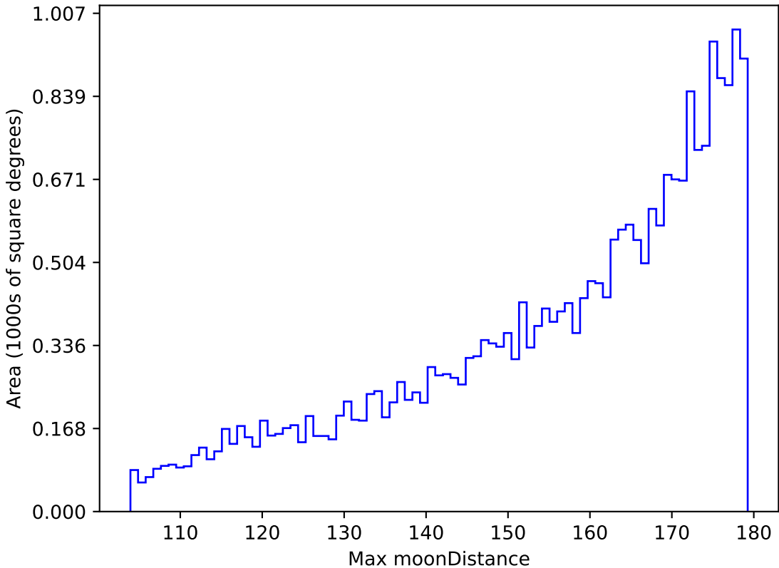
weather_cloudso35v3.4_10yrs All sky i band: Max moonDistance
