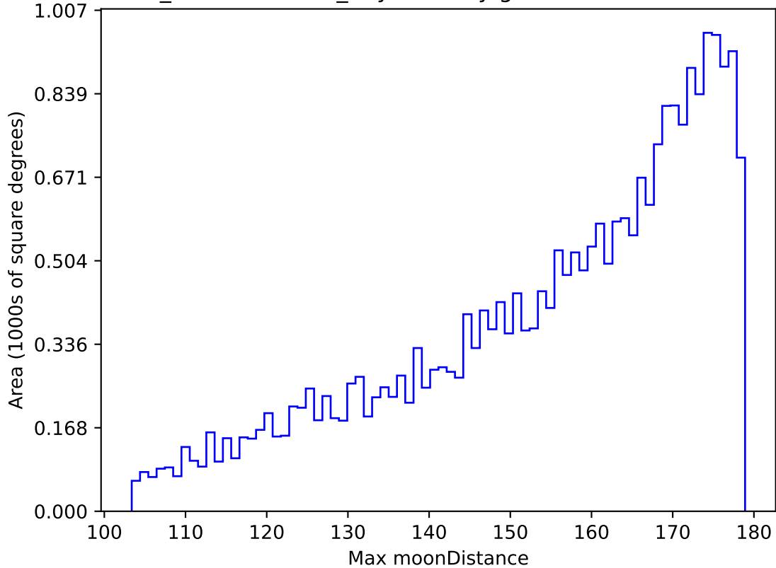
weather_cloudso35v3.4_10yrs All sky g band: Max moonDistance
