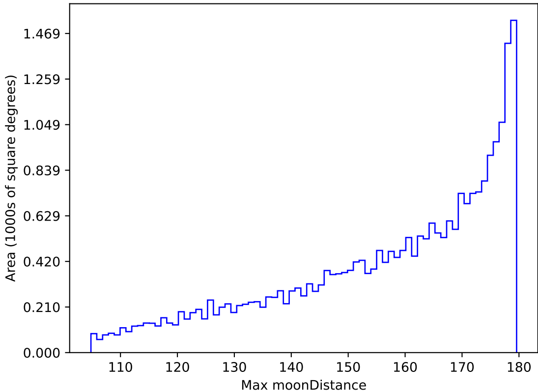
weather_cloudso35v3.4_10yrs All sky all bands: Max moonDistance
