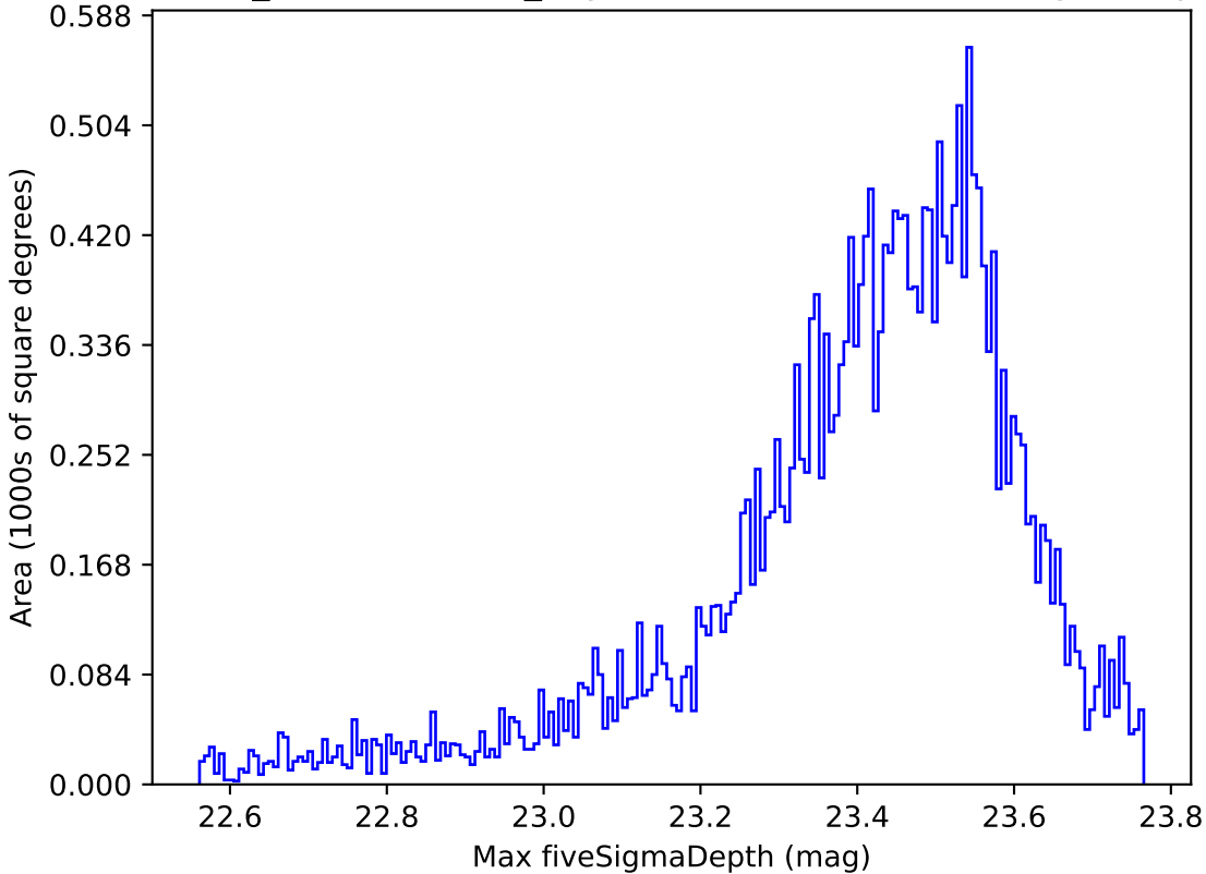
weather_cloudso35v3.4_10yrs Yr 1 z band: Max fiveSigmaDepth
