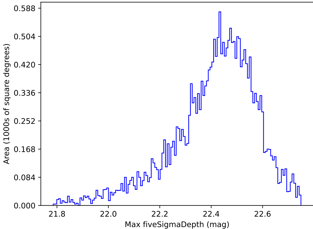
weather_cloudso35v3.4_10yrs Yr 1 y band: Max fiveSigmaDepth
