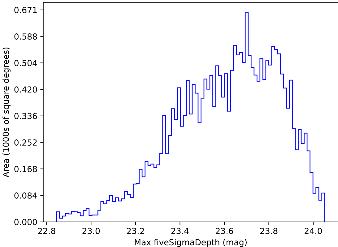
weather_cloudso35v3.4_10yrs Yr 1 u band: Max fiveSigmaDepth
