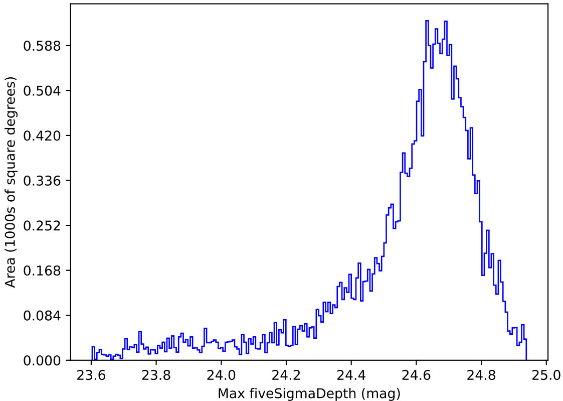
weather_cloudso35v3.4_10yrs Yr 1 r band: Max fiveSigmaDepth
