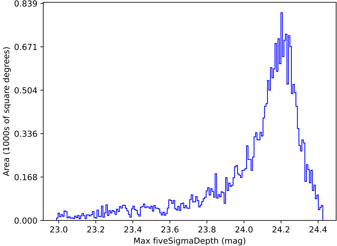
weather_cloudso35v3.4_10yrs Yr 1 i band: Max fiveSigmaDepth
