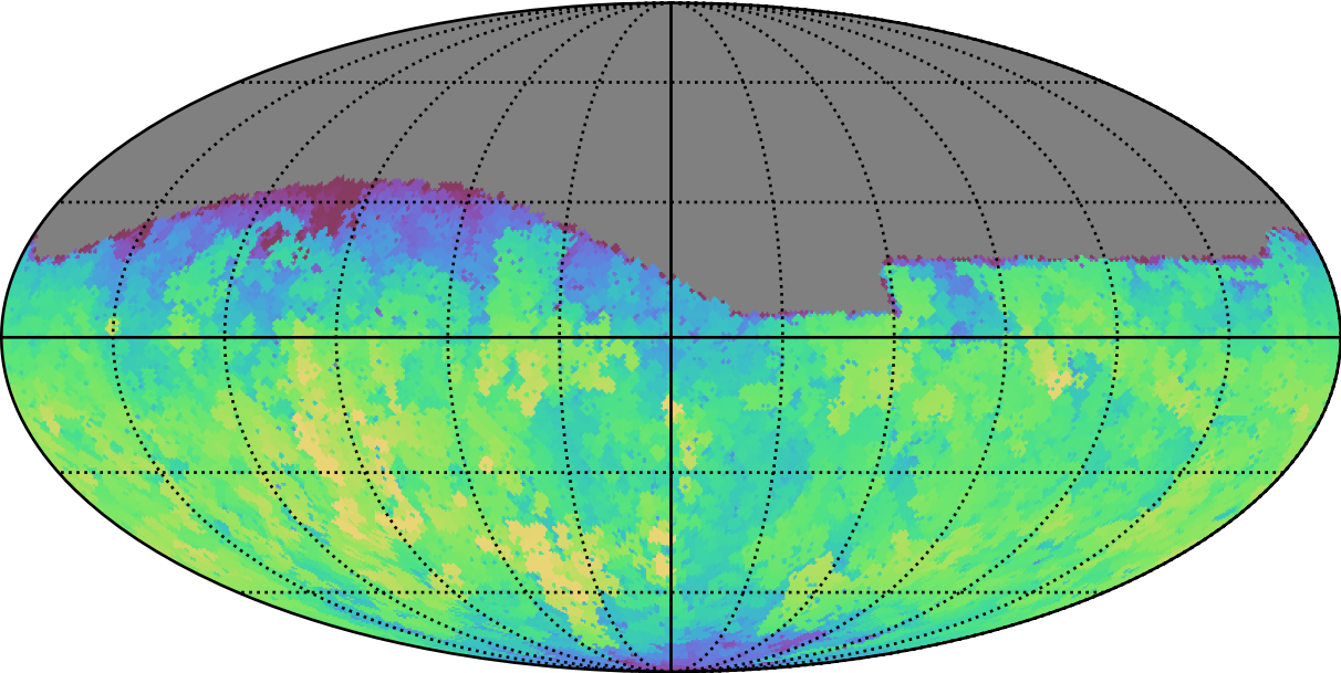
weather_cloudso35v3.4_10yrs Yr 1 all bands: Max fiveSigmaDepth
