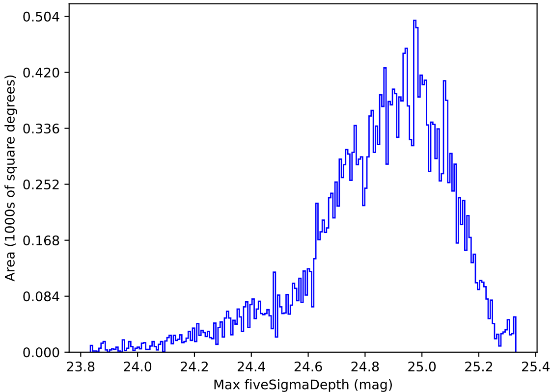
weather_cloudso35v3.4_10yrs Yr 1 all bands: Max fiveSigmaDepth
