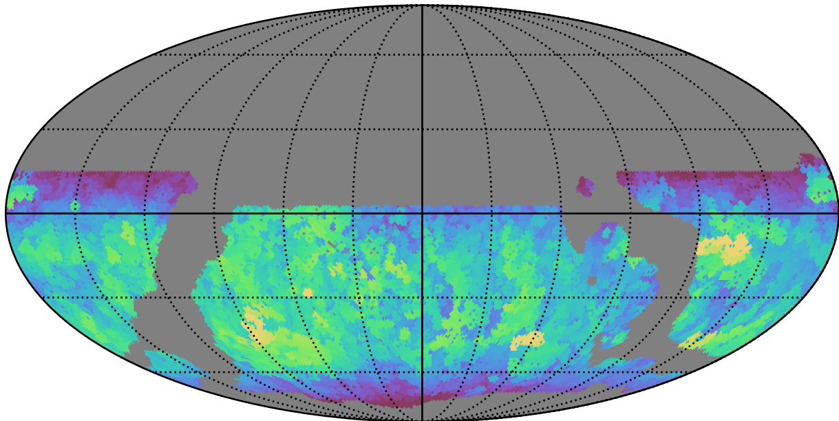
weather_cloudso35v3.4_10yrs WFD y band: Max fiveSigmaDepth
