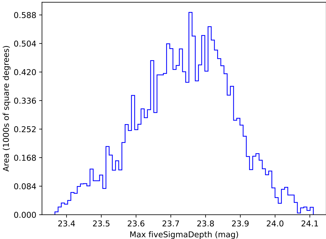
weather_cloudso35v3.4_10yrs WFD u band: Max fiveSigmaDepth
