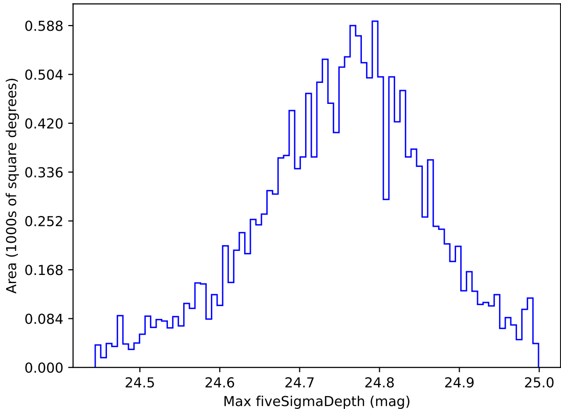
weather_cloudso35v3.4_10yrs WFD r band: Max fiveSigmaDepth
