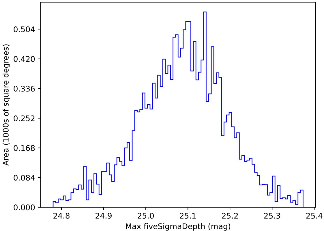
weather_cloudso35v3.4_10yrs WFD g band: Max fiveSigmaDepth
