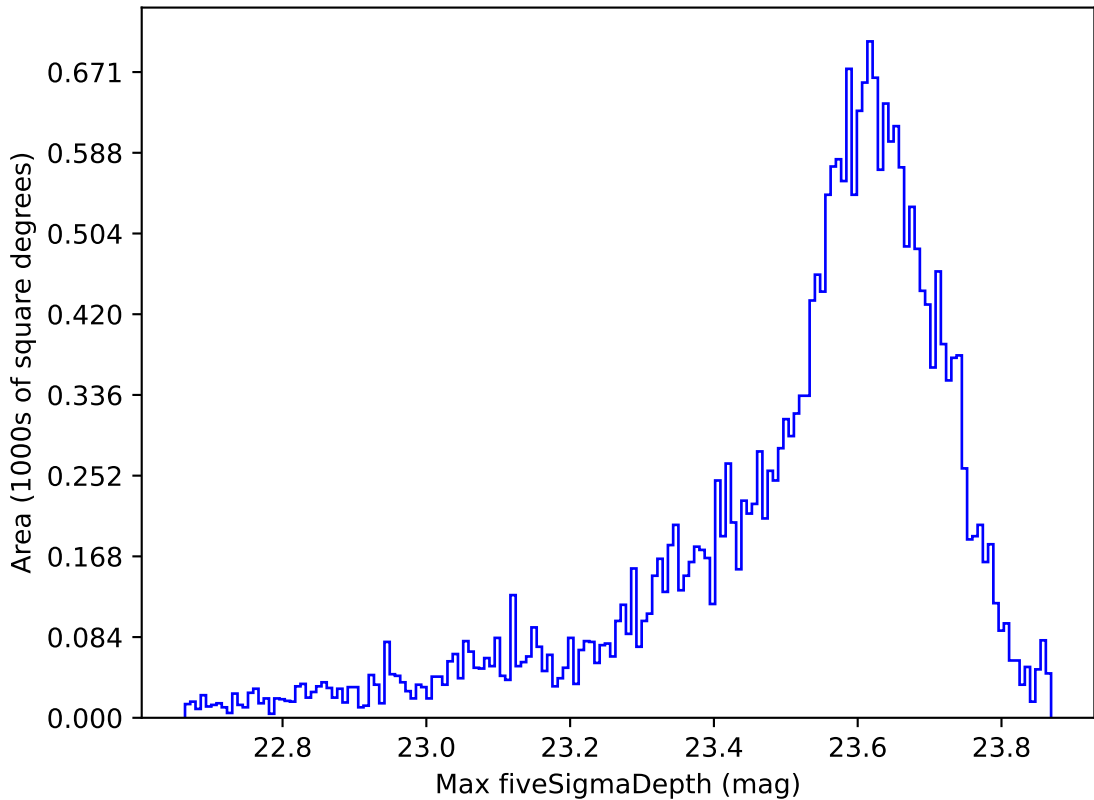
weather_cloudso35v3.4_10yrs All sky z band: Max fiveSigmaDepth
