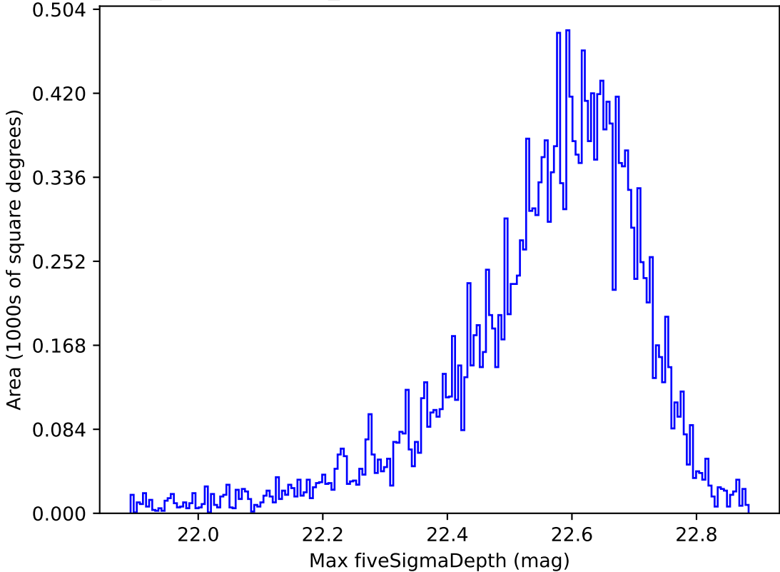
weather_cloudso35v3.4_10yrs All sky y band: Max fiveSigmaDepth
