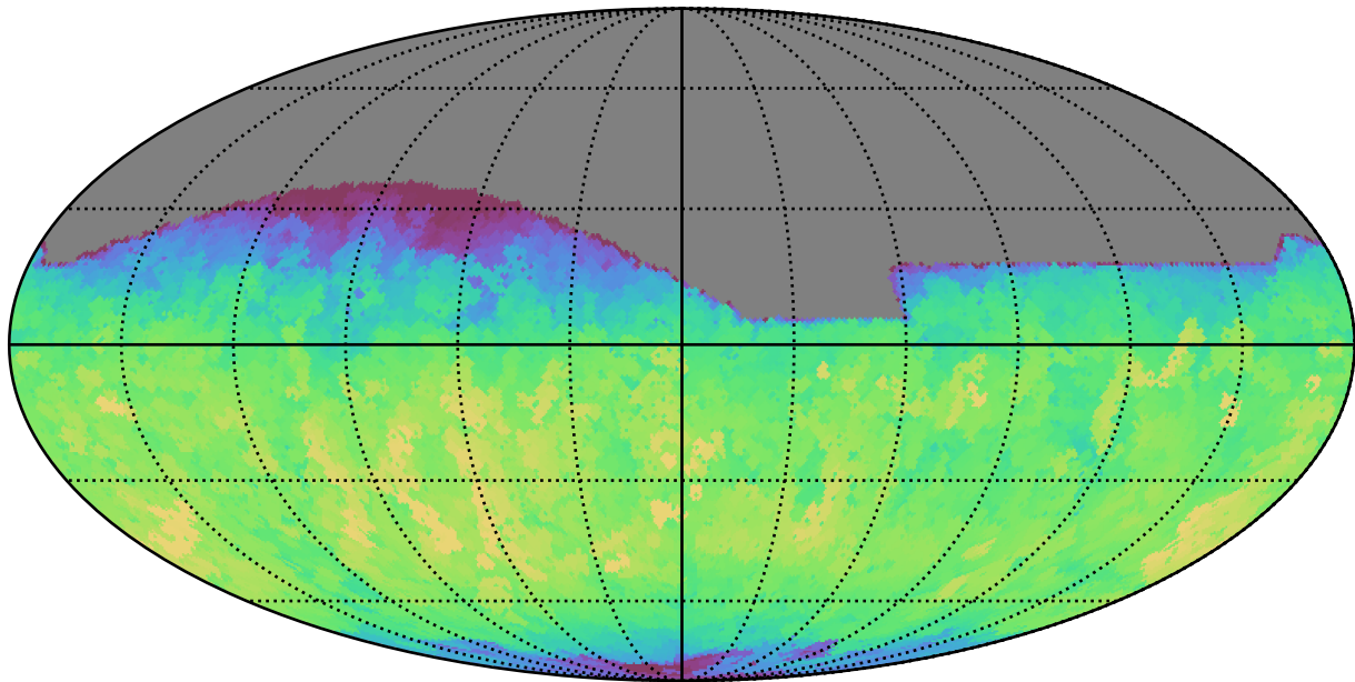
weather_cloudso35v3.4_10yrs All sky r band: Max fiveSigmaDepth
