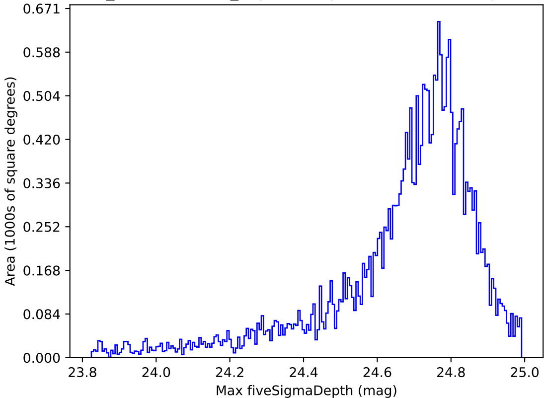
weather_cloudso35v3.4_10yrs All sky r band: Max fiveSigmaDepth
