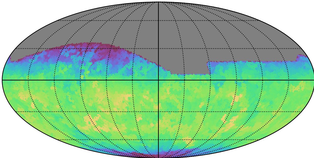
weather_cloudso35v3.4_10yrs All sky i band: Max fiveSigmaDepth
