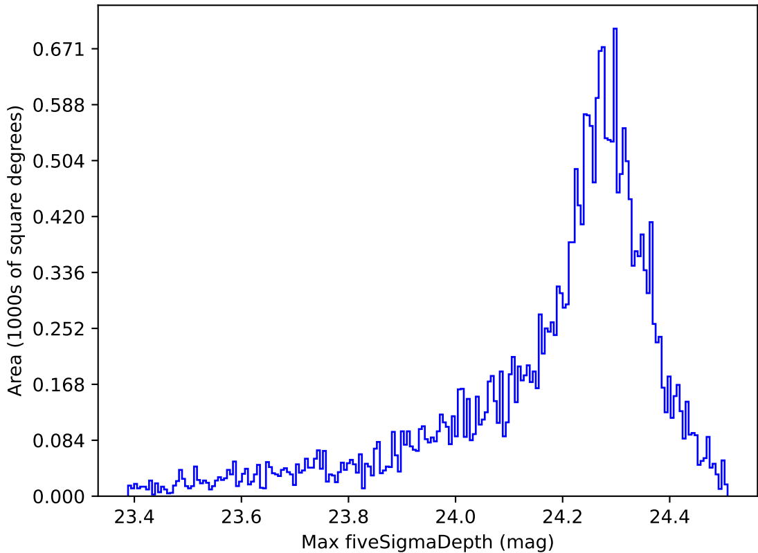
weather_cloudso35v3.4_10yrs All sky i band: Max fiveSigmaDepth
