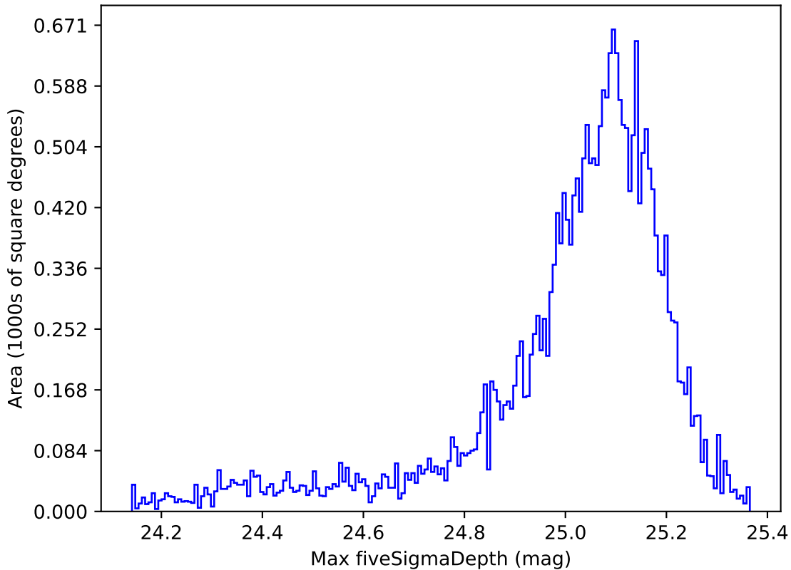
weather_cloudso35v3.4_10yrs All sky g band: Max fiveSigmaDepth
