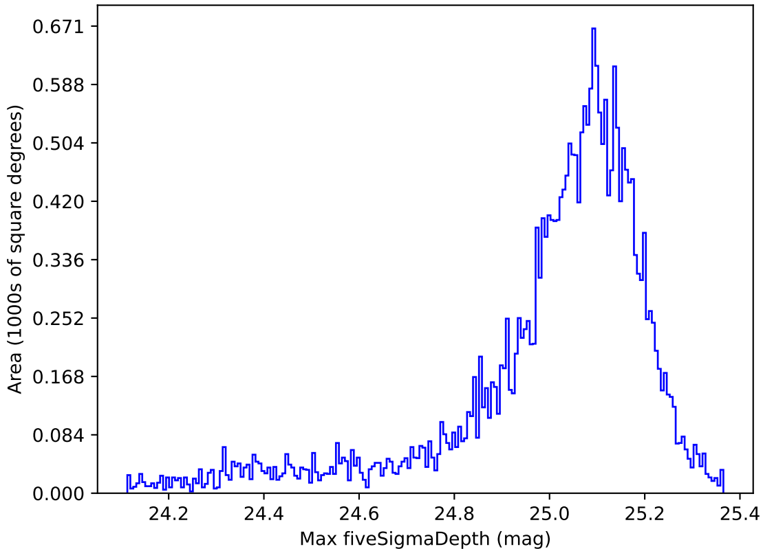
weather_cloudso35v3.4_10yrs All sky all bands: Max fiveSigmaDepth
