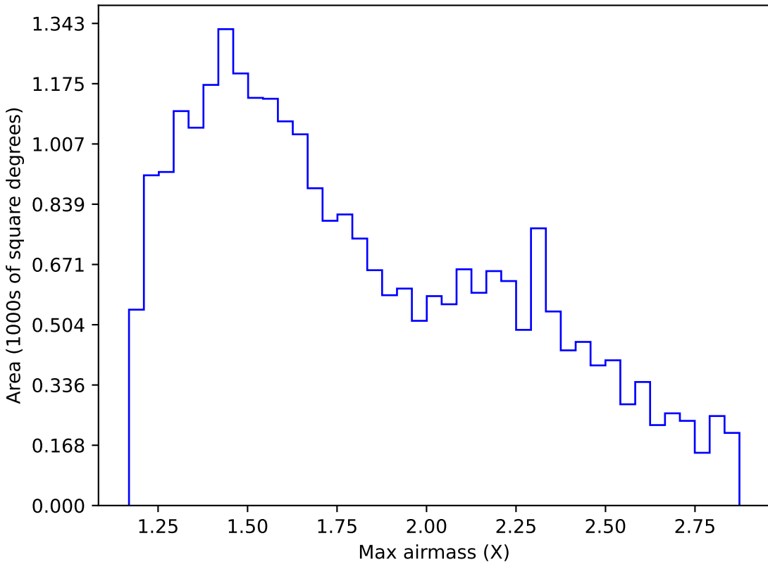
weather_cloudso35v3.4_10yrs Yr 1 z band: Max airmass
