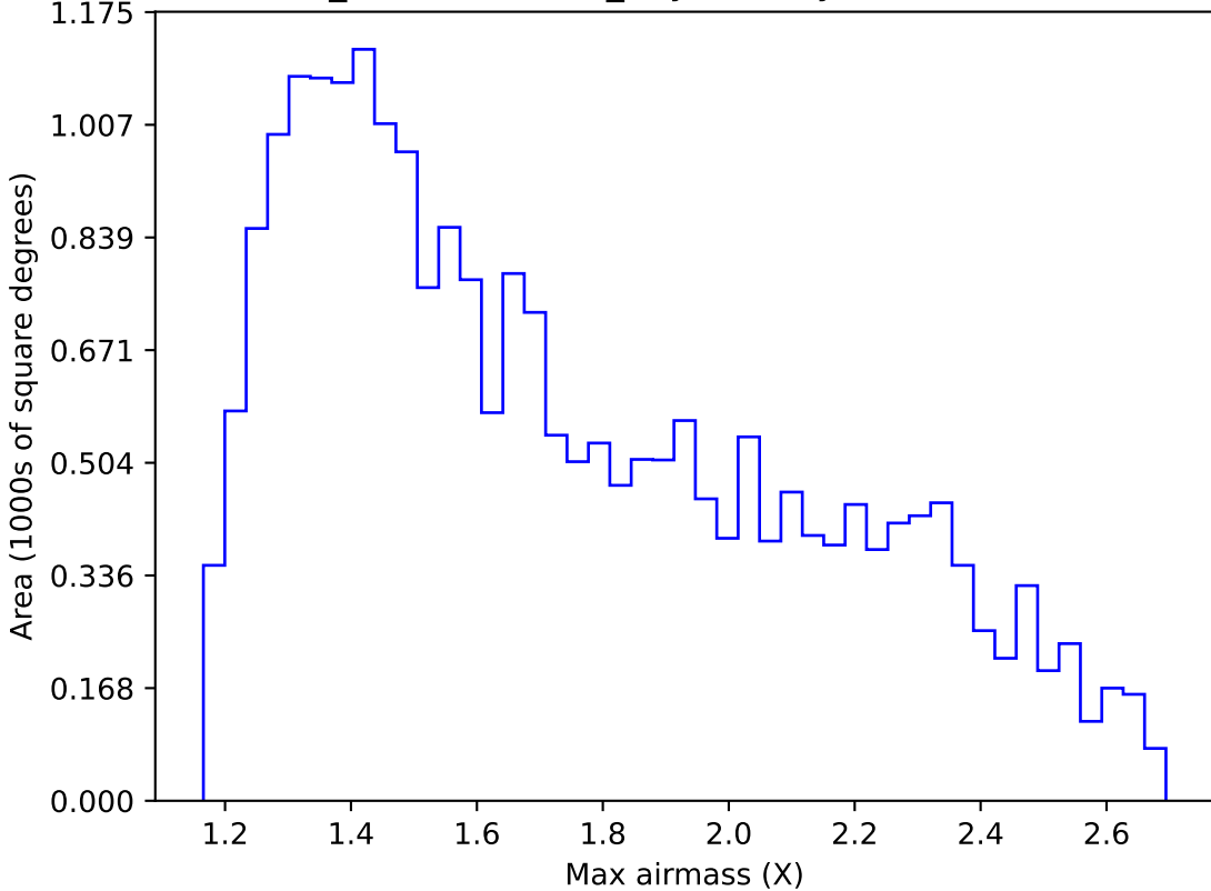
weather_cloudso35v3.4_10yrs Yr 1 y band: Max airmass
