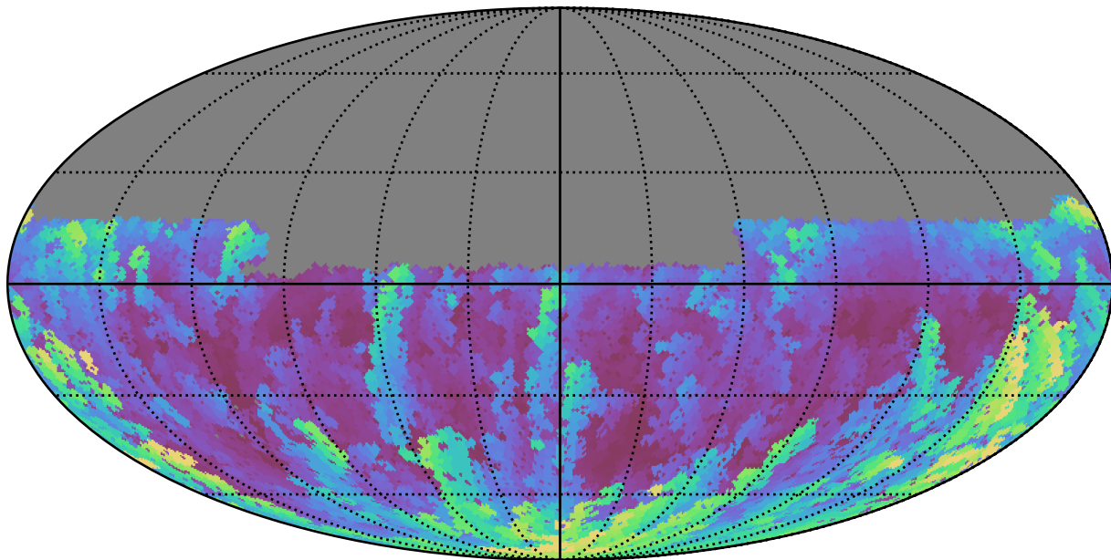
weather_cloudso35v3.4_10yrs Yr 1 u band: Max airmass
