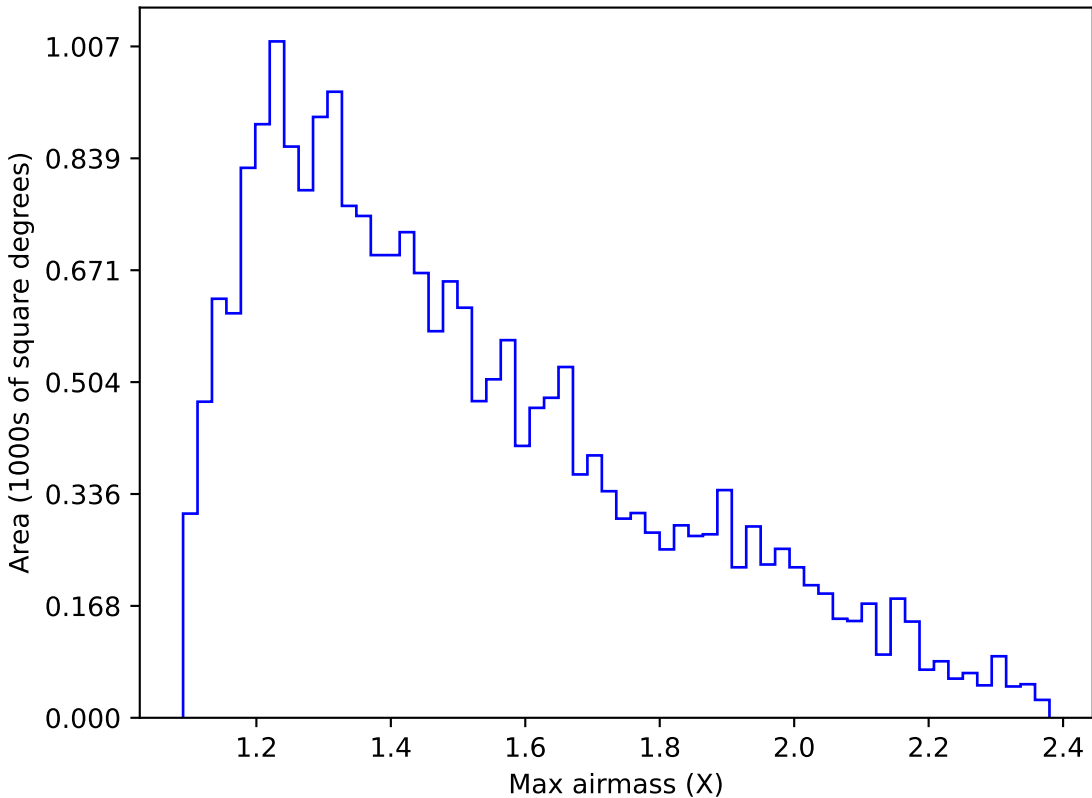
weather_cloudso35v3.4_10yrs Yr 1 u band: Max airmass
