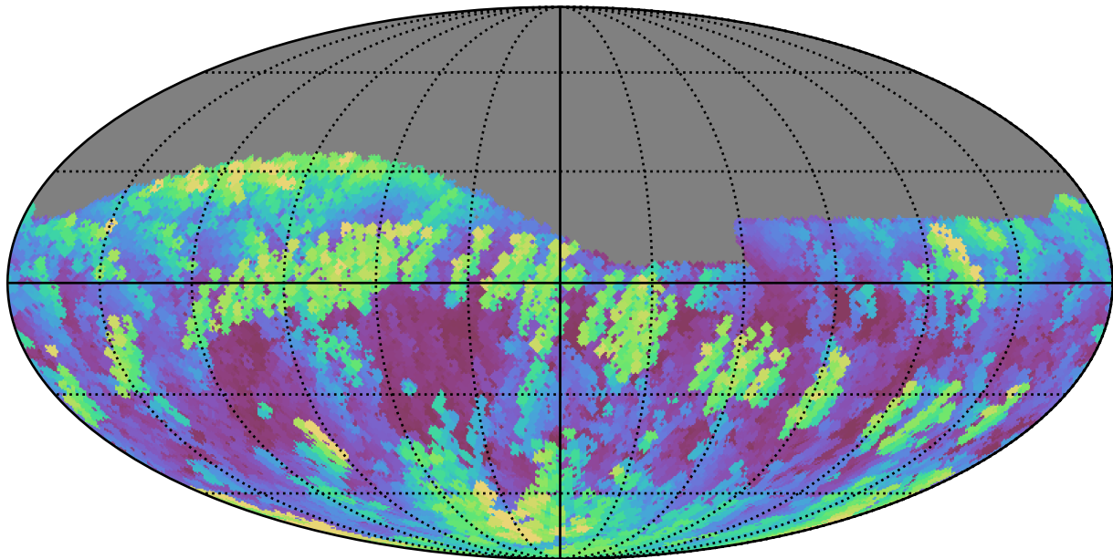
weather_cloudso35v3.4_10yrs Yr 1 r band: Max airmass
