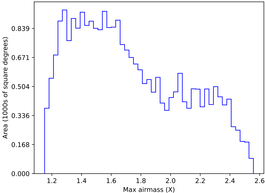
weather_cloudso35v3.4_10yrs Yr 1 r band: Max airmass
