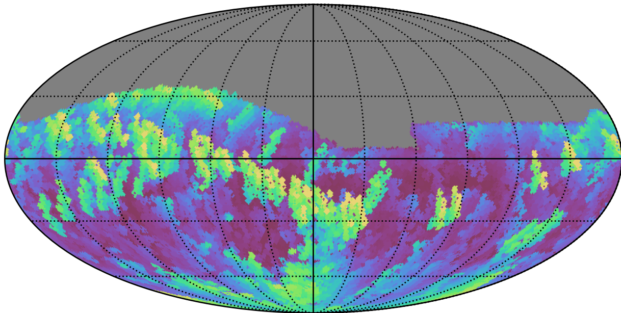
weather_cloudso35v3.4_10yrs Yr 1 i band: Max airmass
