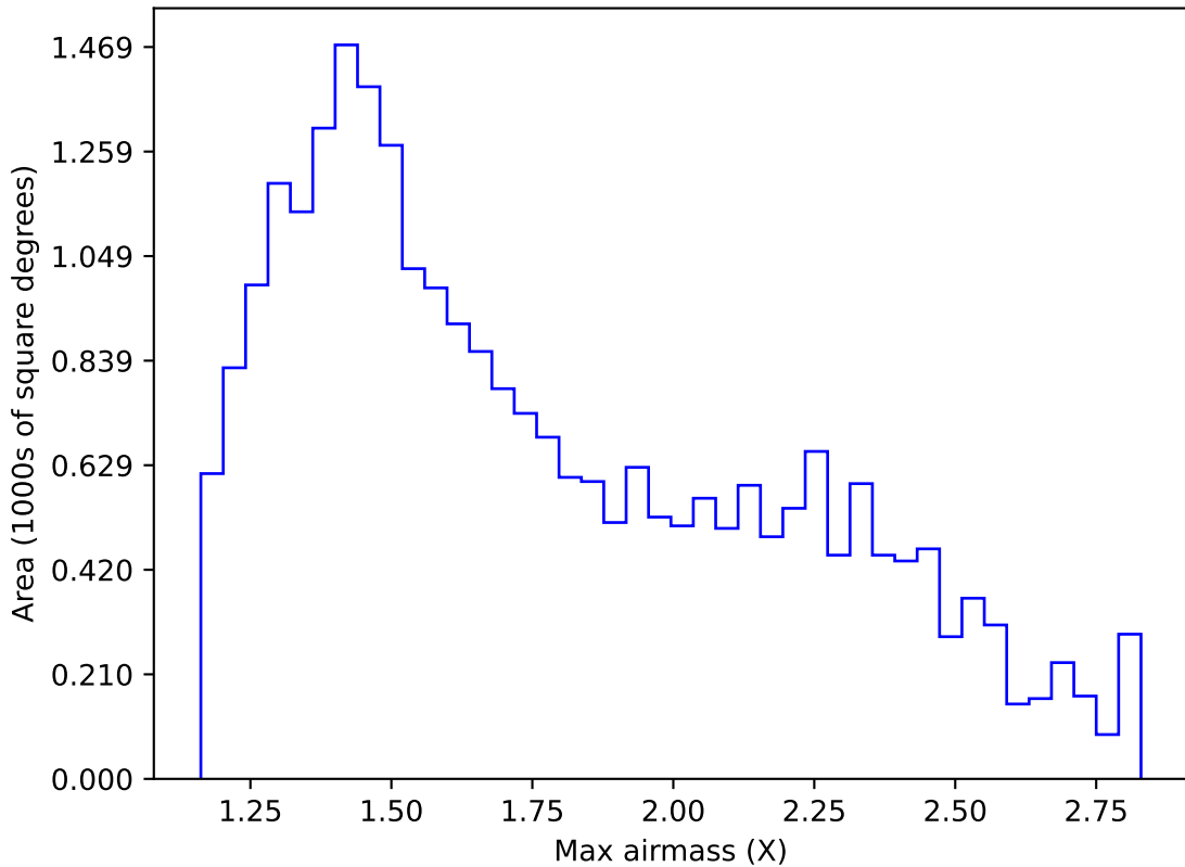
weather_cloudso35v3.4_10yrs Yr 1 i band: Max airmass
