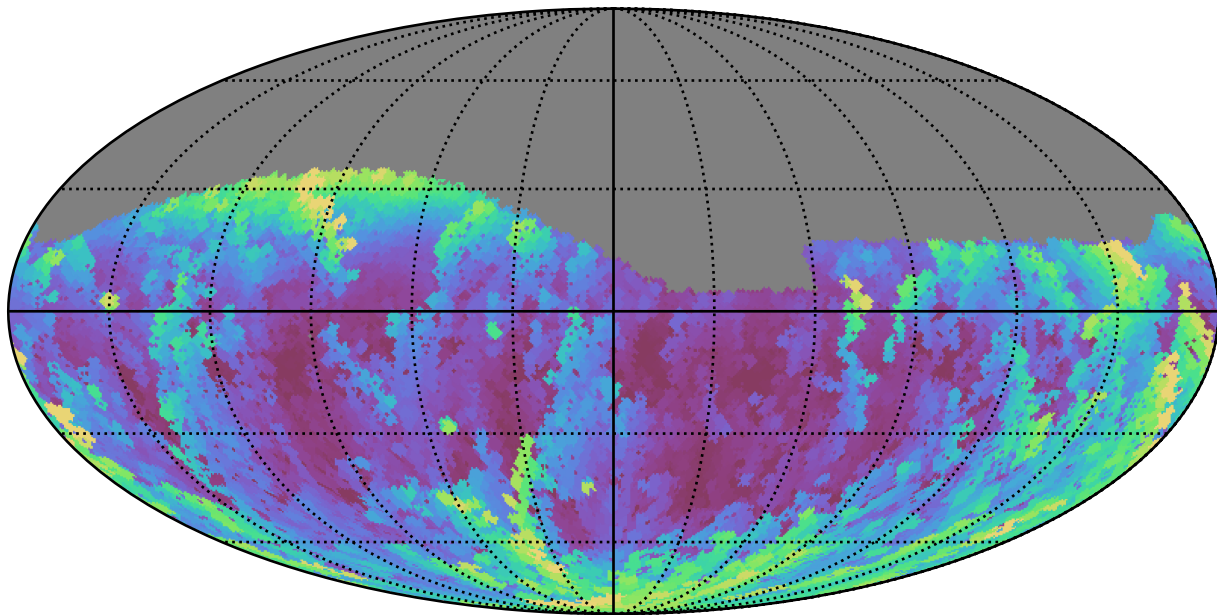
weather_cloudso35v3.4_10yrs Yr 1 g band: Max airmass
